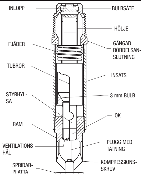
FIGUR 2 SERIES DS-1, 1\"/>
